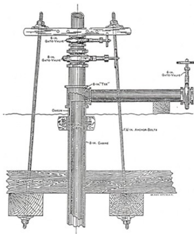
METHOD EMPLOYED TO CLOSE THE LUCAS GUSHER
